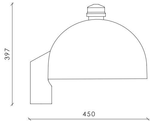
Dimensions with NEMA socket
