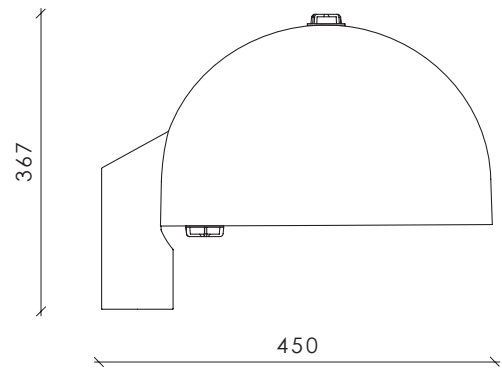
Dimensions with 2 Zhaga connectors
