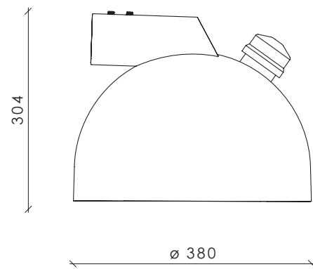
Dimensions with NEMA socket
