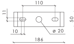
Mounting console
