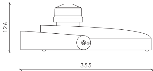
Dimensions with NEMA
