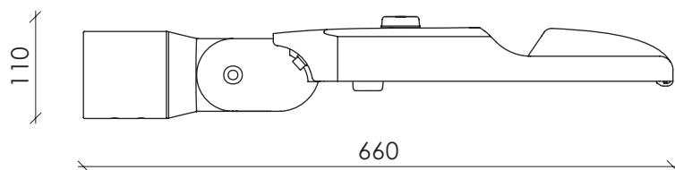
Dimensions with 2 Zhaga connectors
