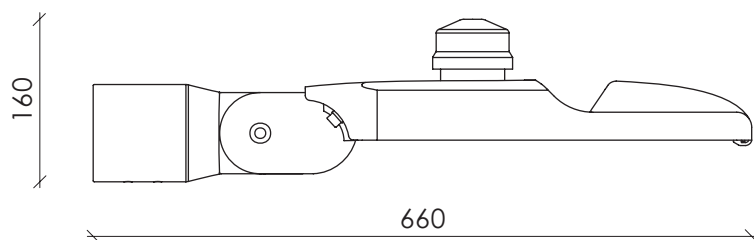
Dimensions with NEMA socket
