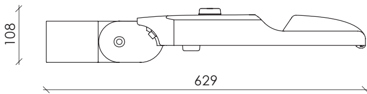
Dimensions with 2 Zhaga connectors
