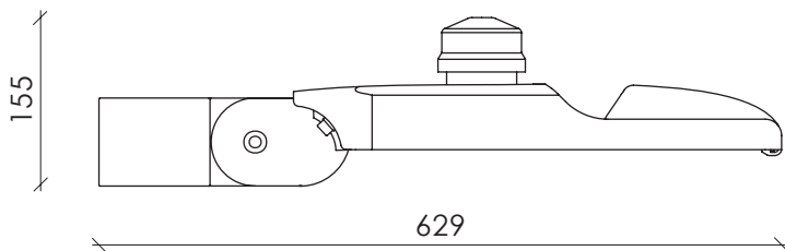
Dimensions with NEMA socket
